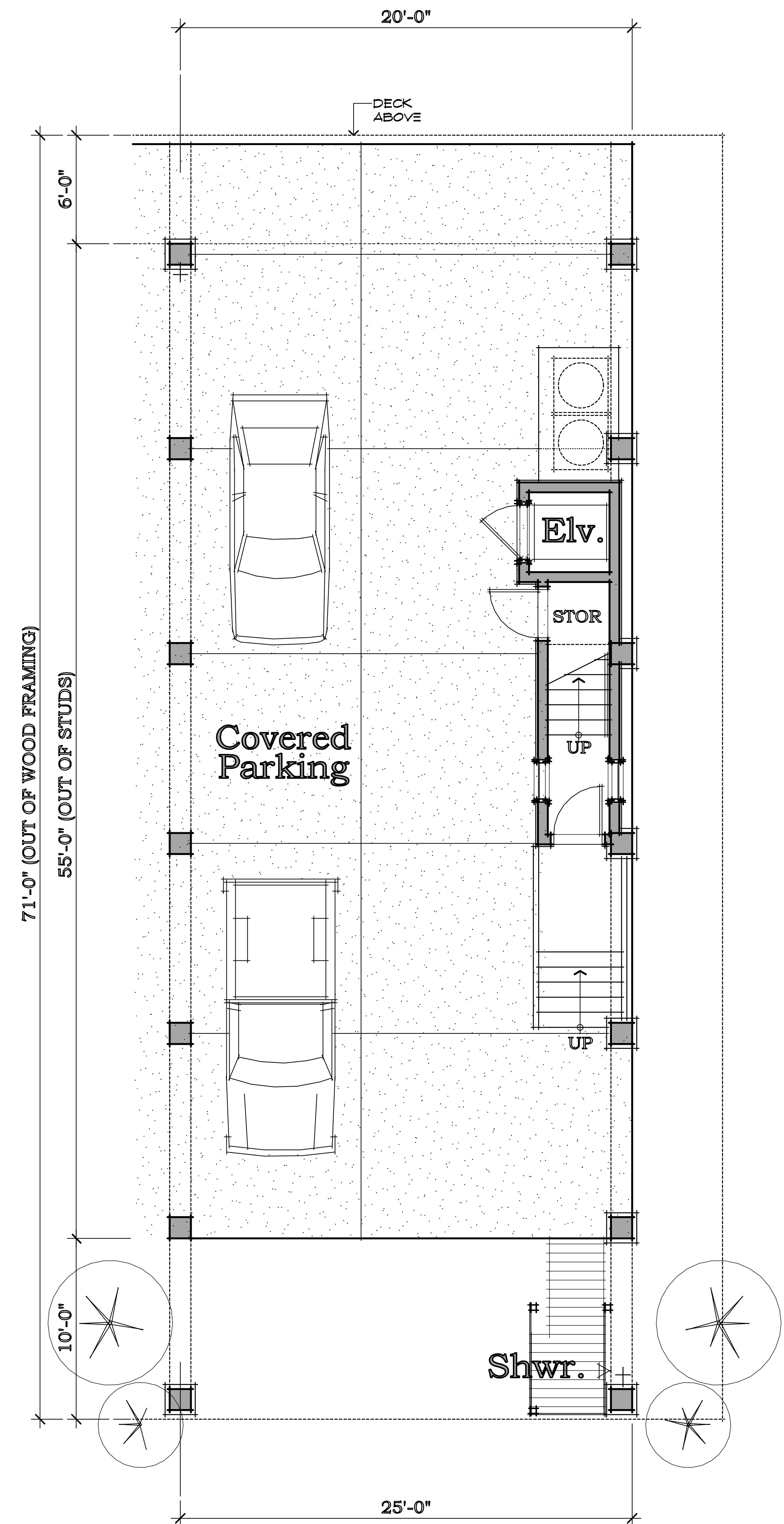
Ground Floor Plan TYPICAL 25' UNIT PLAN
