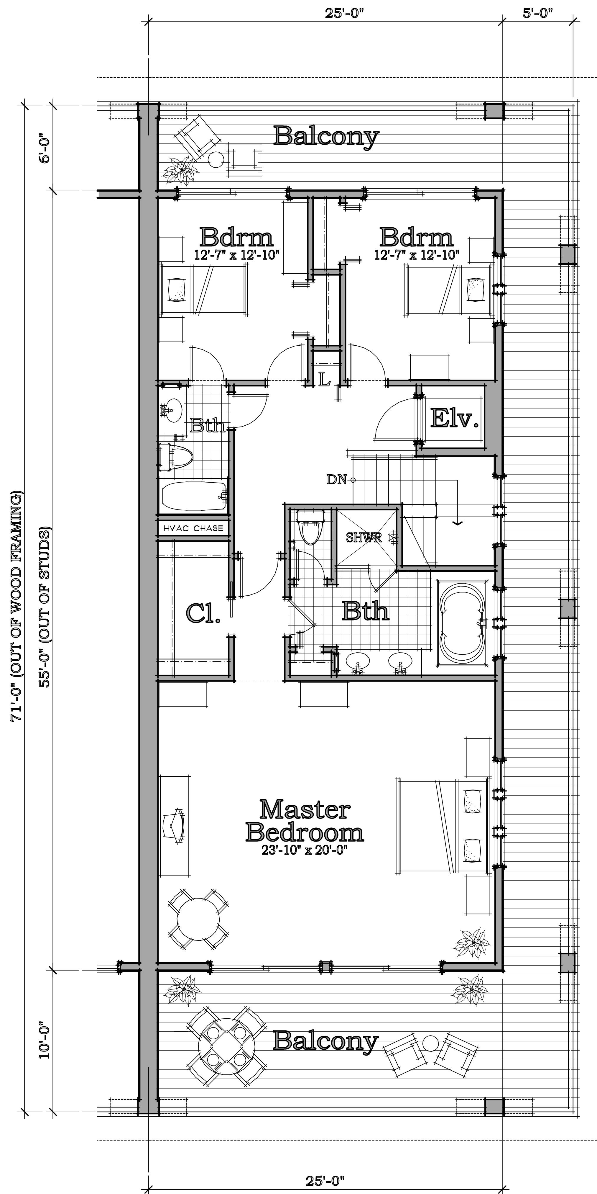
Second Floor Plan TYPICAL 25' UNIT PLAN
