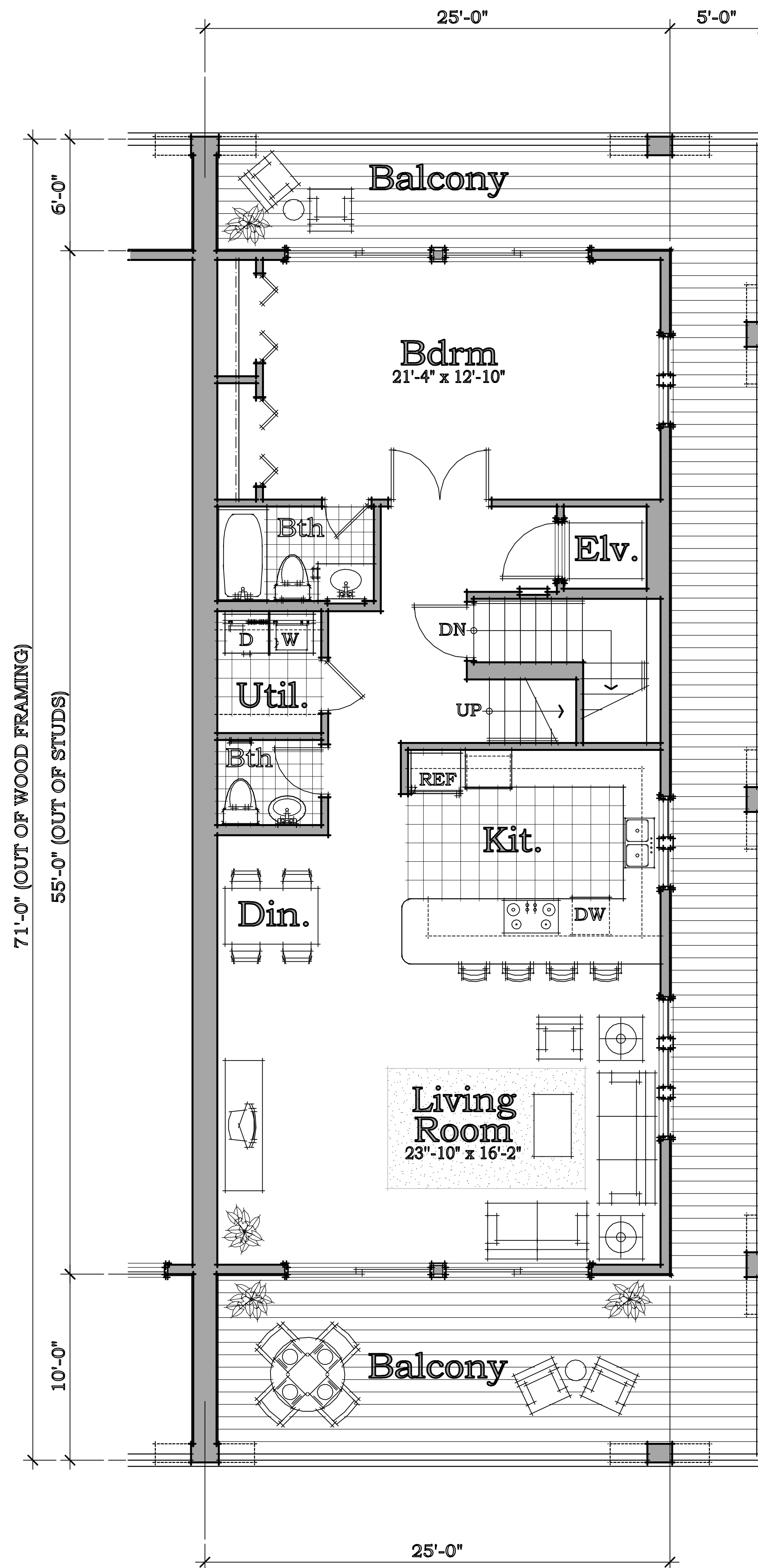
First Floor Plan TYPICAL 25' UNIT PLAN
