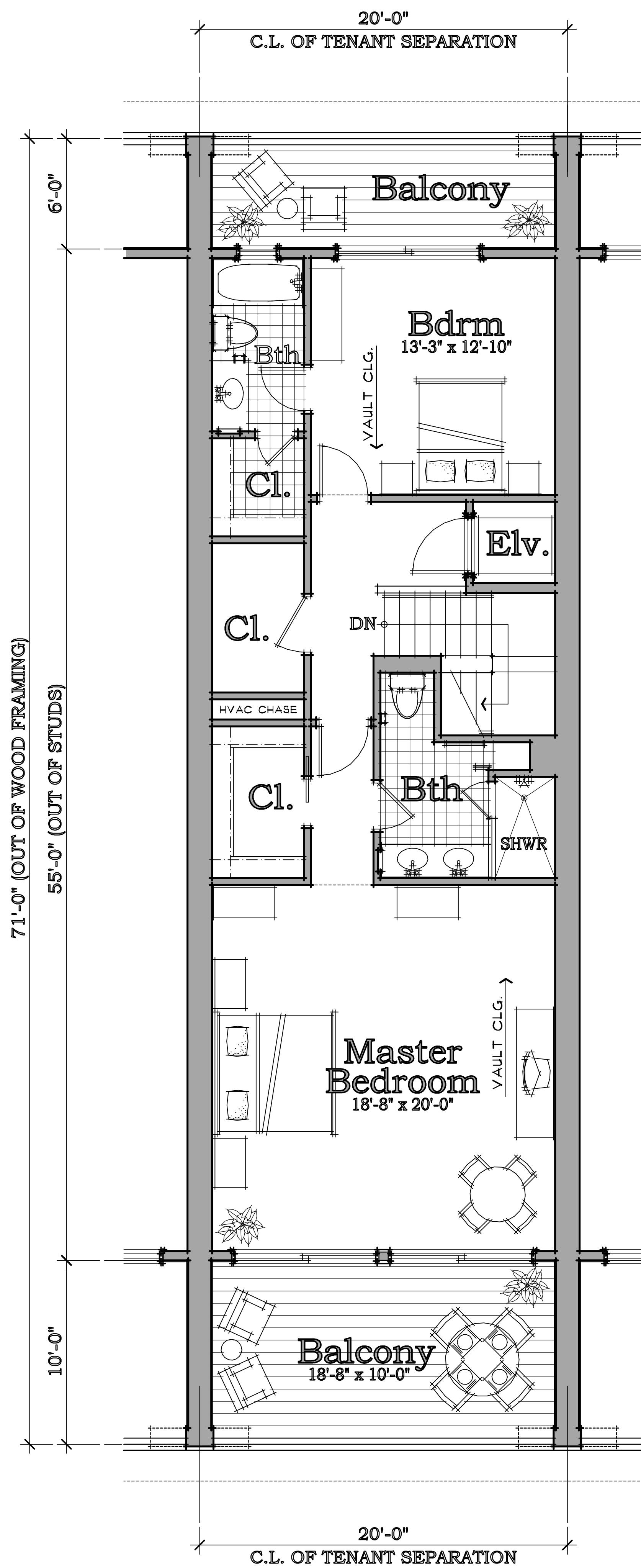
Second Floor Plan TYPICAL 20' UNIT PLAN
