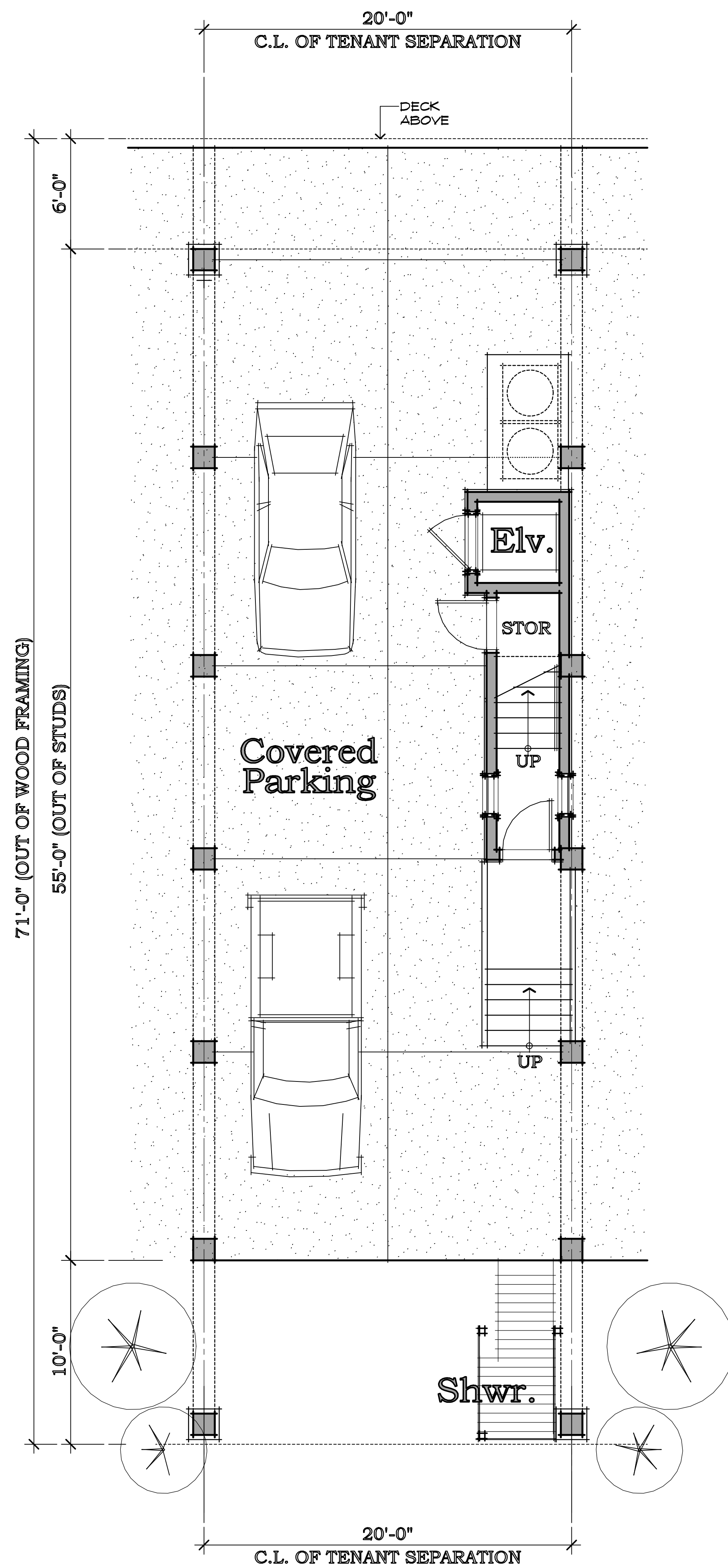
Ground Floor Plan TYPICAL 20' UNIT PLAN
